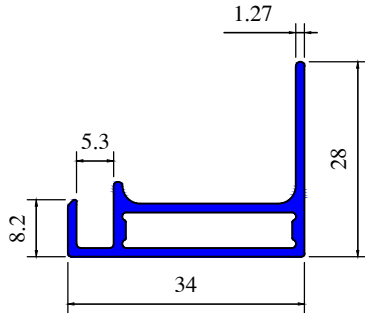
Section No 1450
