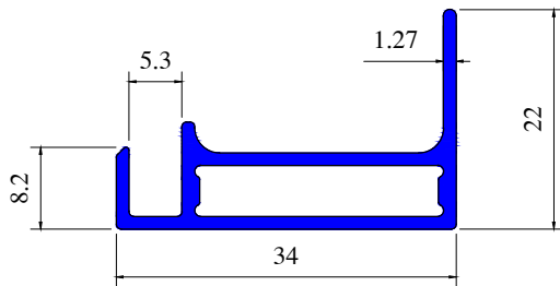
Section No 1431
