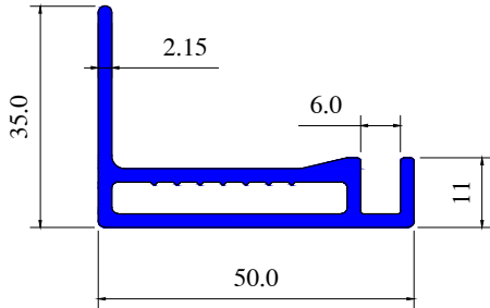
Section No 1409
