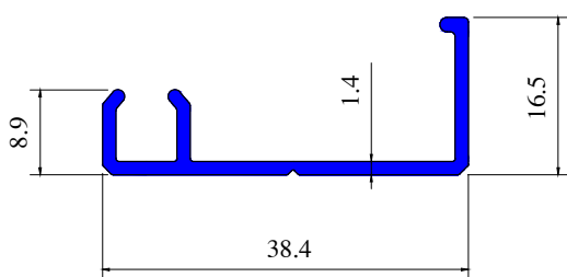
Section No 1404
