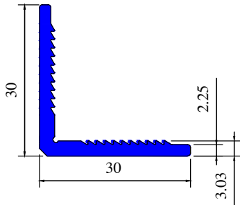
Section No 1459
