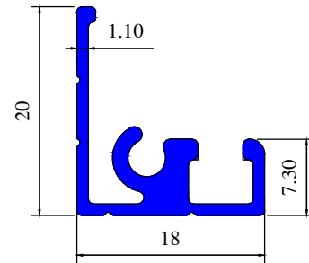
Section No 1464
