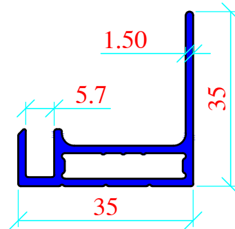
Section No 1473
