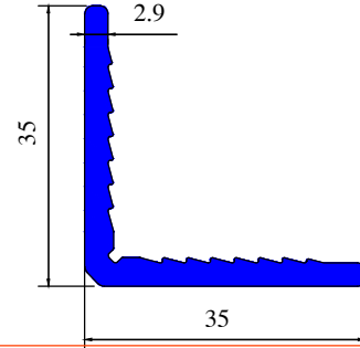
Section No 1463
