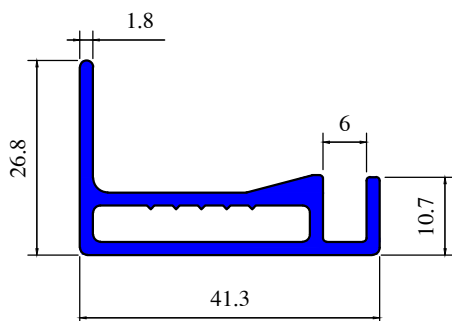
Section No 1443
