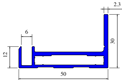
Section No 1439
