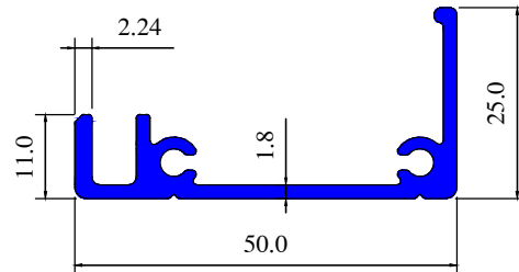
Section No 1449
