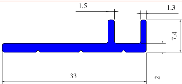
Section No 1403
