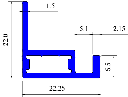
Section No 1401
