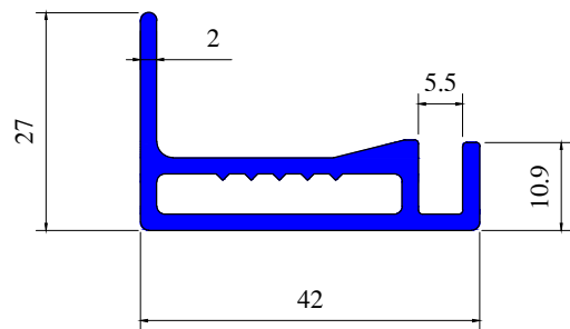
Section No 1420
