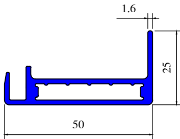
Section No 1452
