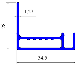
Section No 1469
