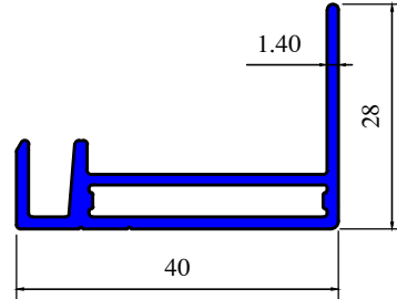
Section No 1471
