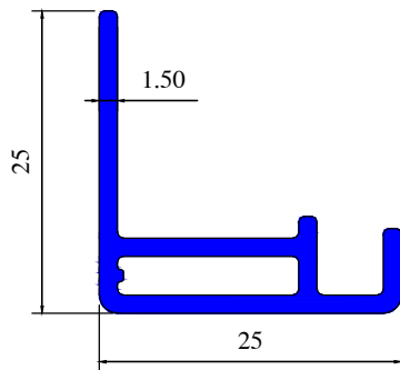
Section No 1461
