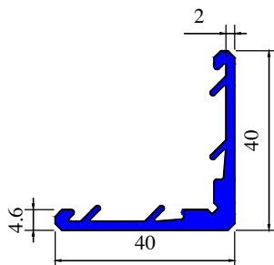
Section No 1453
