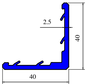
Section No 1470
