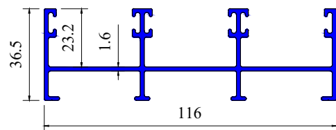
3 TRACK FRAME TOP&SIDE
