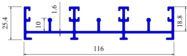
3 TRACK FRAME BOTTOM
