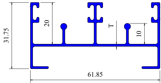
2 TRACK FRAME BOTTOM
