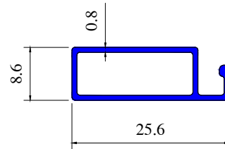
Section No 4008
