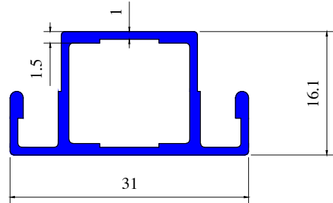
Section No 4008
