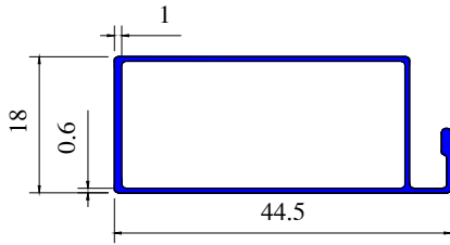
Section No 4029
