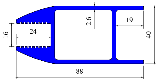
GLAZING PATTI
