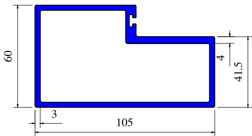
Section No 4737
