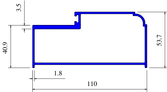
Section No 4730
