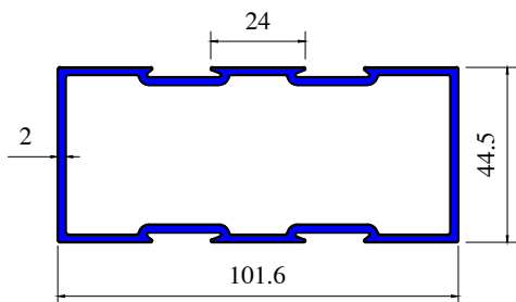
Section No 4737
