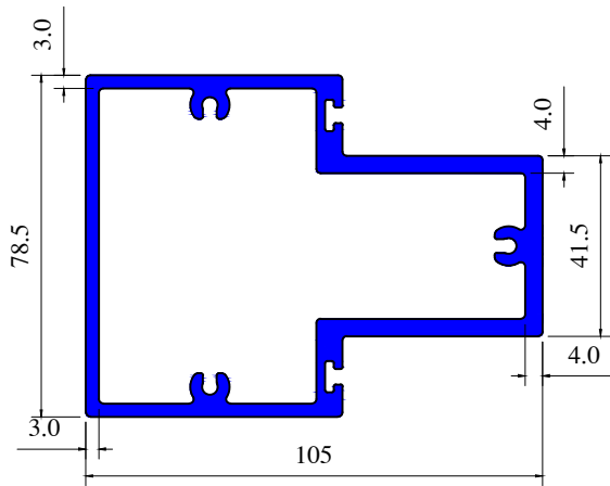
Section No 4730
